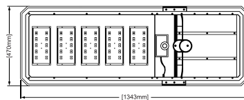
Dimension ( mm )
